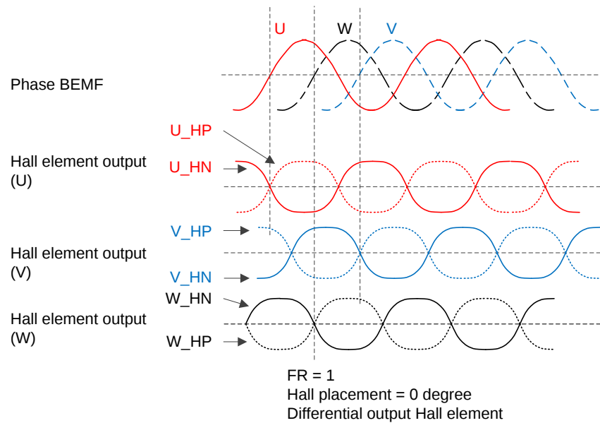
图 24. Correspondence Between Motor BEMF and Hall Signal ( FR = 1 , 0^\circ Placement)
