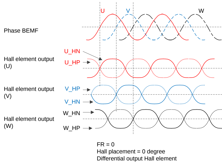
图 25. Correspondence Between Motor BEMF and Hall Signal ( FR = 0 , 0^\circ Placement)
