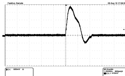
图 7-19. 10BASE-Tc Link Pulse Waveform
