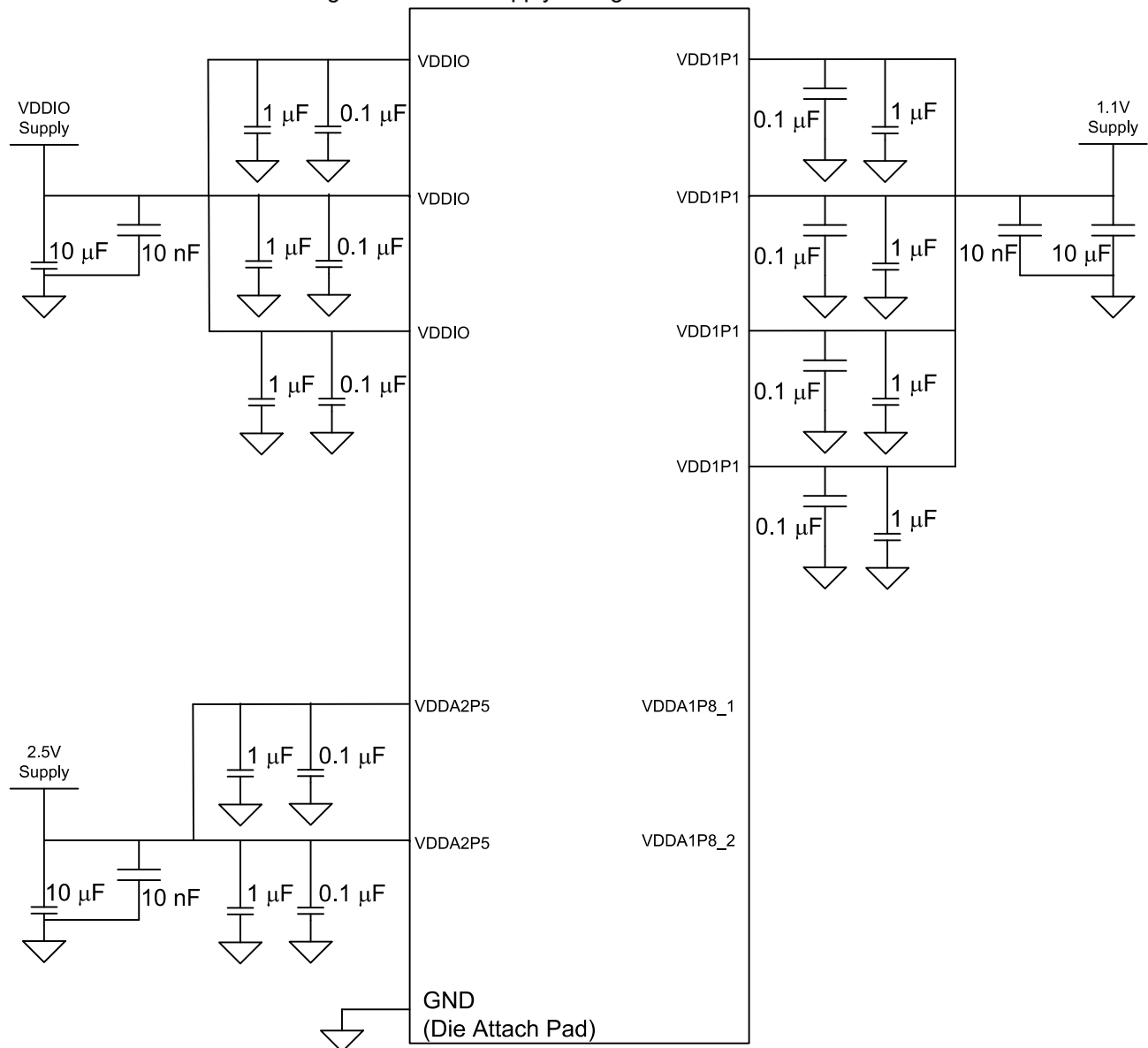
图 9-1. Two-Supply Configuration
