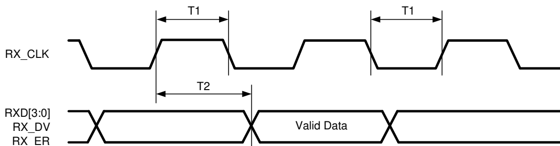
图 6-4. 100-Mbps MII Receive Timing
