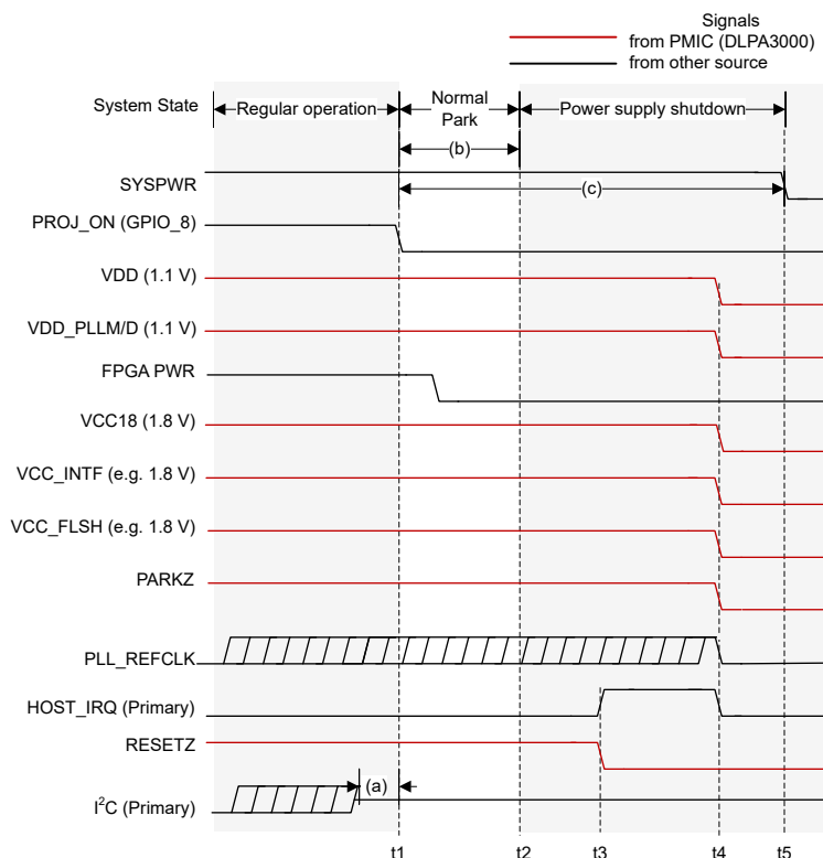
图 9-2. DLPC3437 Normal Power-Down
