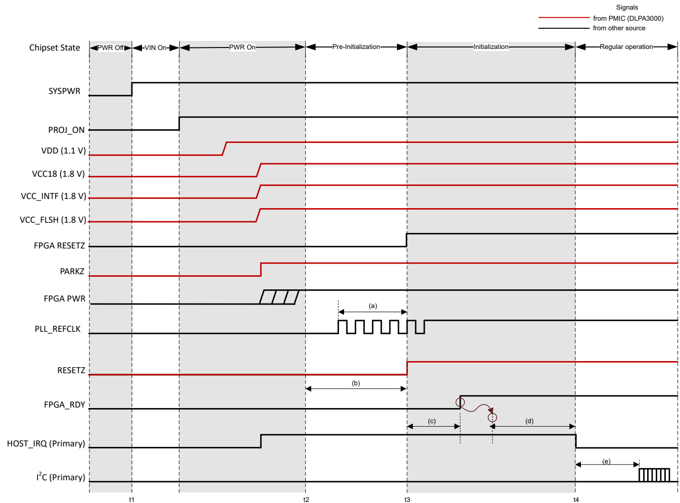
图 9-1. DLPC3437 Power-Up Timing
