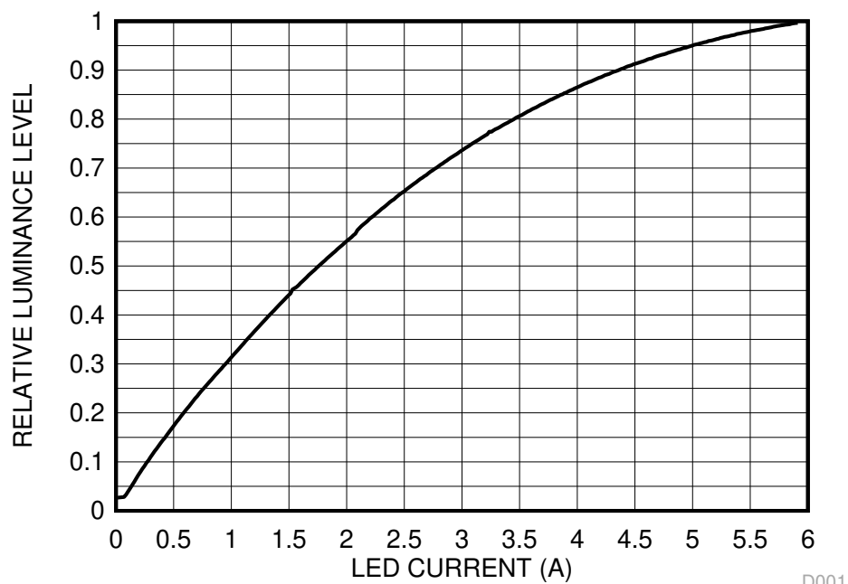
图 8-2. Typical Luminance vs Current
