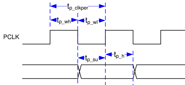
图 6-8. Parallel Interface General Timing
