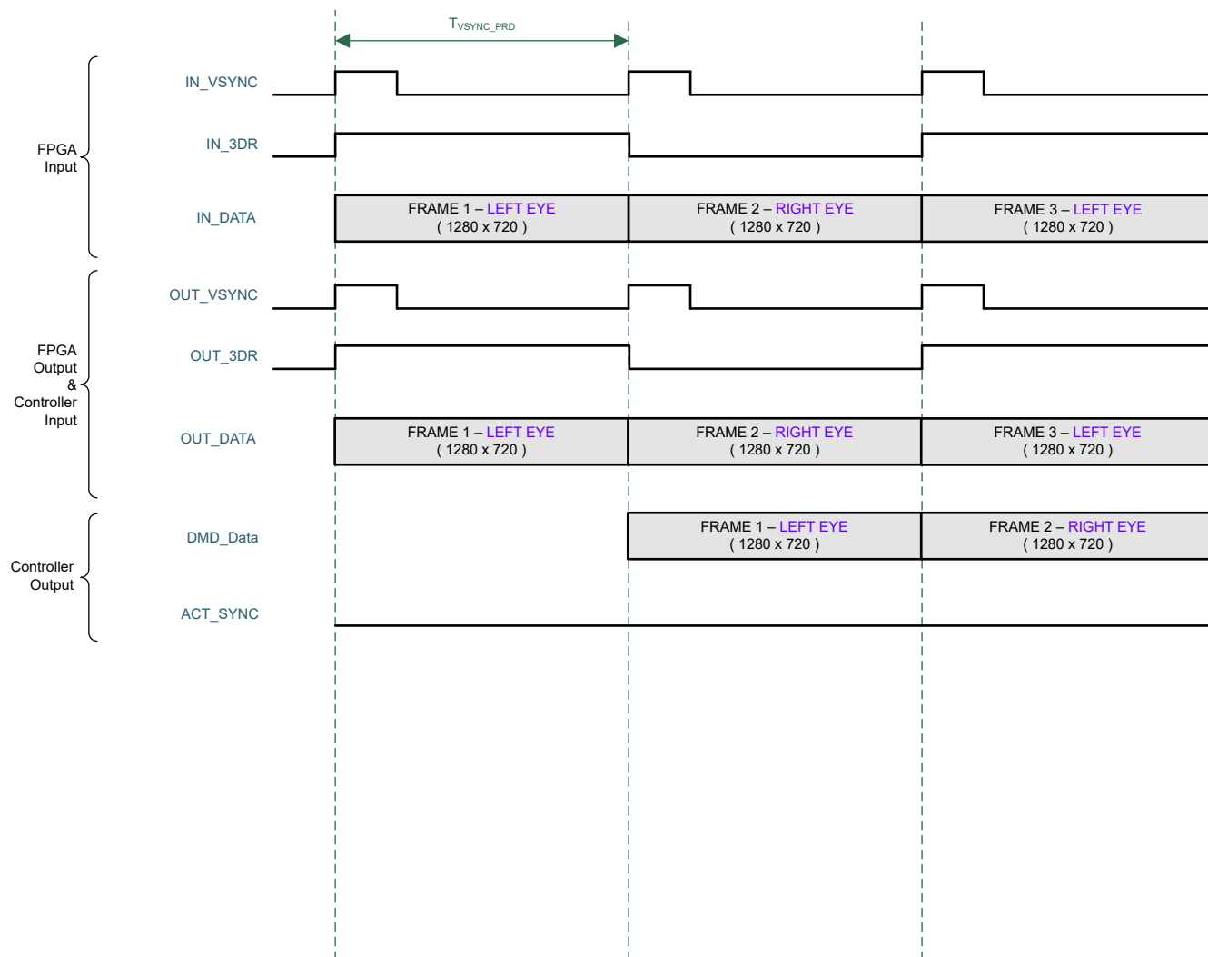
图 7-3. DLPC3437 3D Frame and Signal Timing
