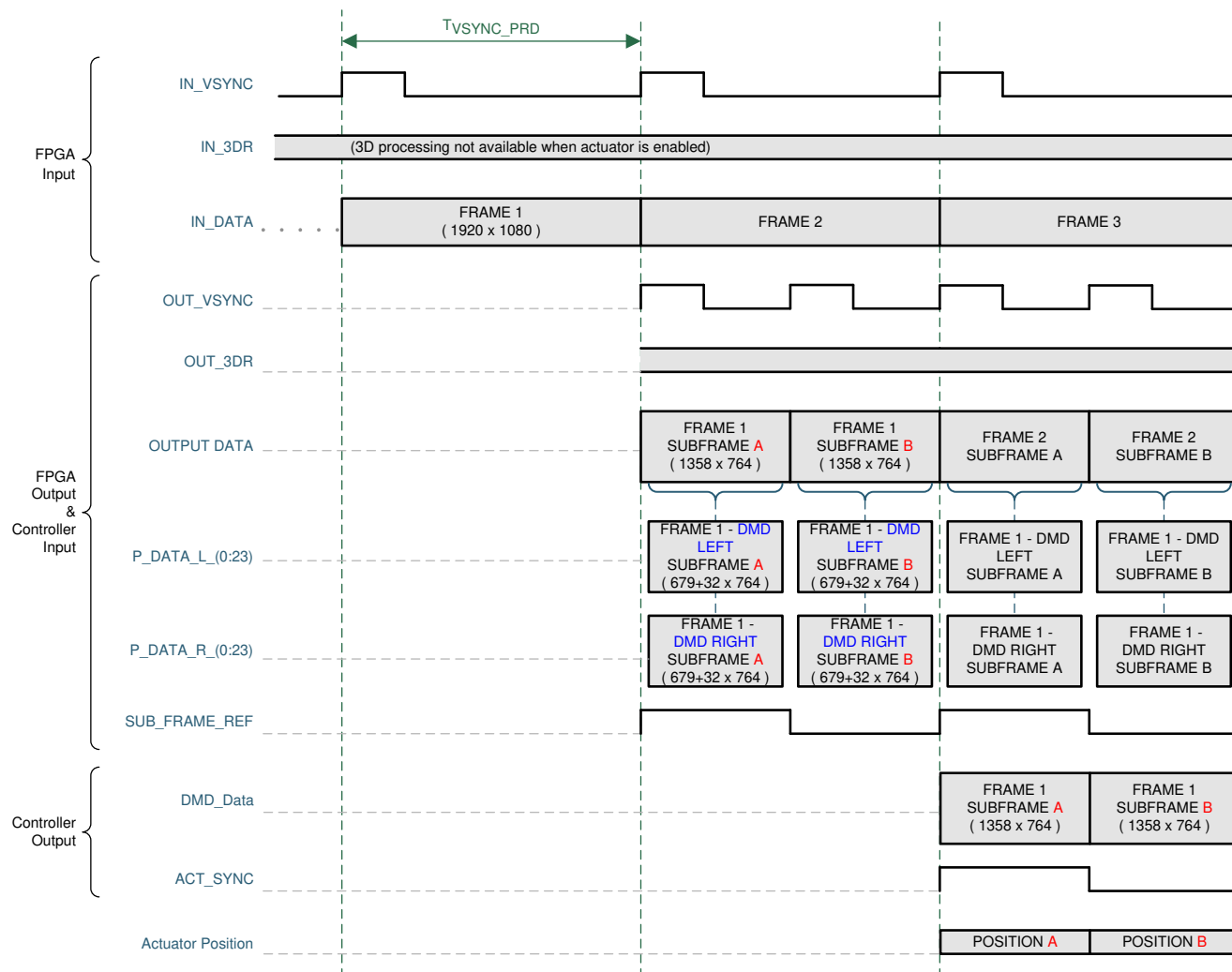
图 7-2. DLPC3437 2D Actuator Frame and Signal Timing
