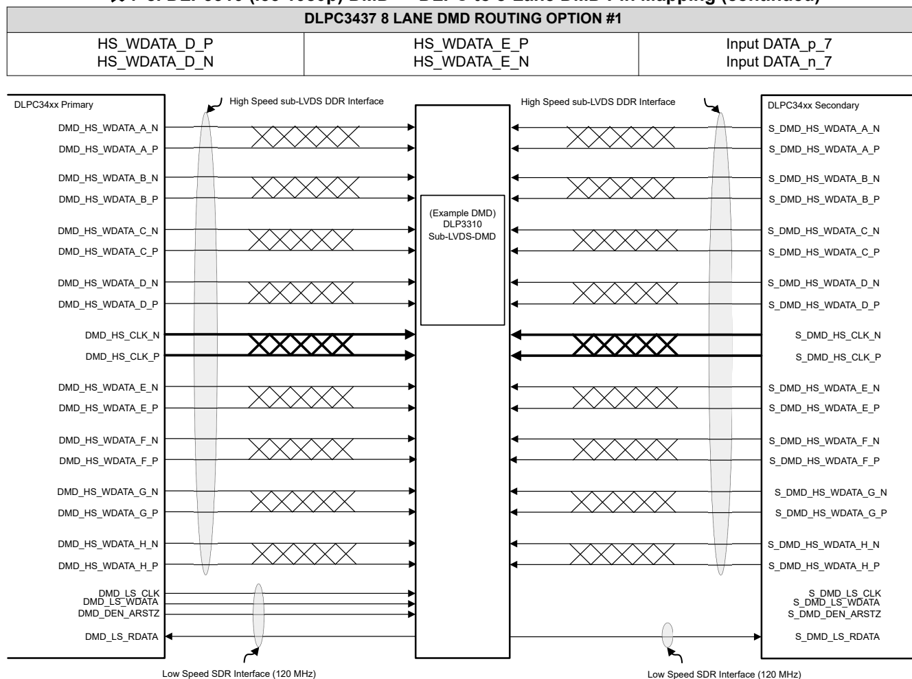
图 7-12. DLP3310 (.33 1080p) DMD Interface Example (Option 1 and 2)
