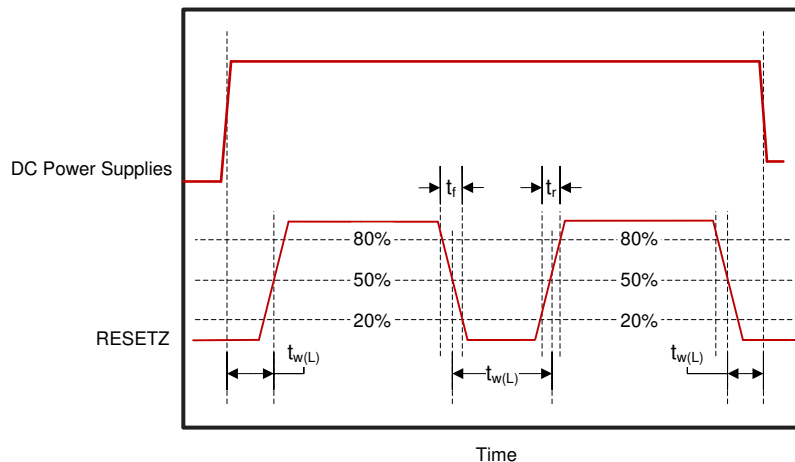
图 5-6. Power-Up and Power-Down RESETZ Timing
