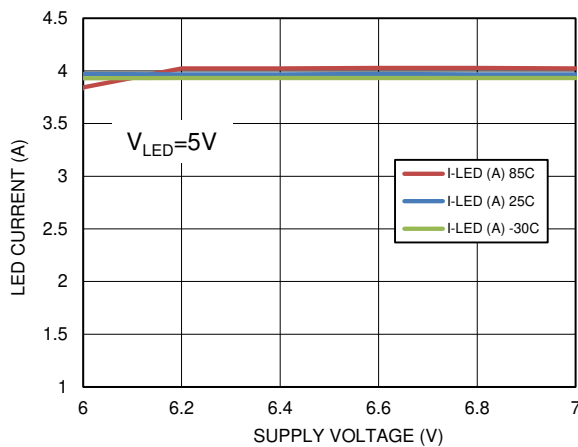
图 8-11. 4-A Led Current at V_{LED} = 5\text{ V}
