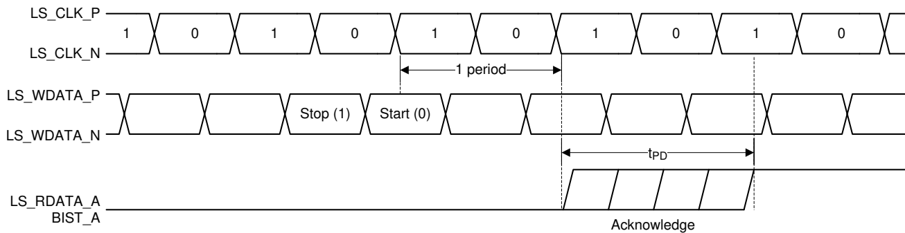
图 5-2. Switching Characteristics
