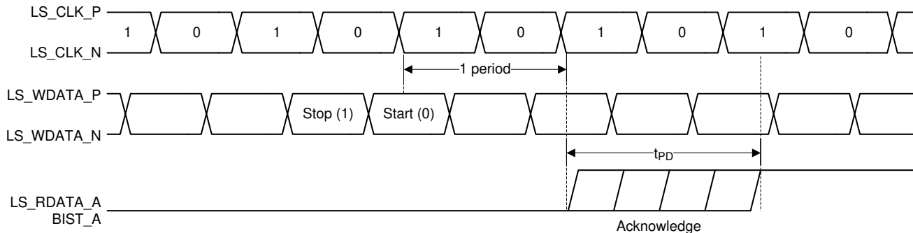
图 5-2. Switching Characteristics
