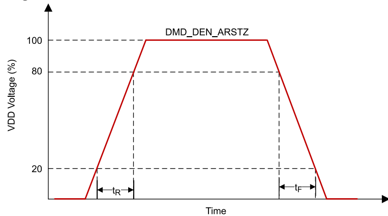
图 5-2. LPSDR Input Rise and Fall Slew Rate
