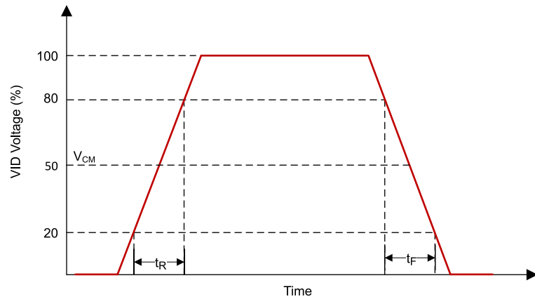
图 5-3. SubLVDS Input Rise and Fall Slew Rate
