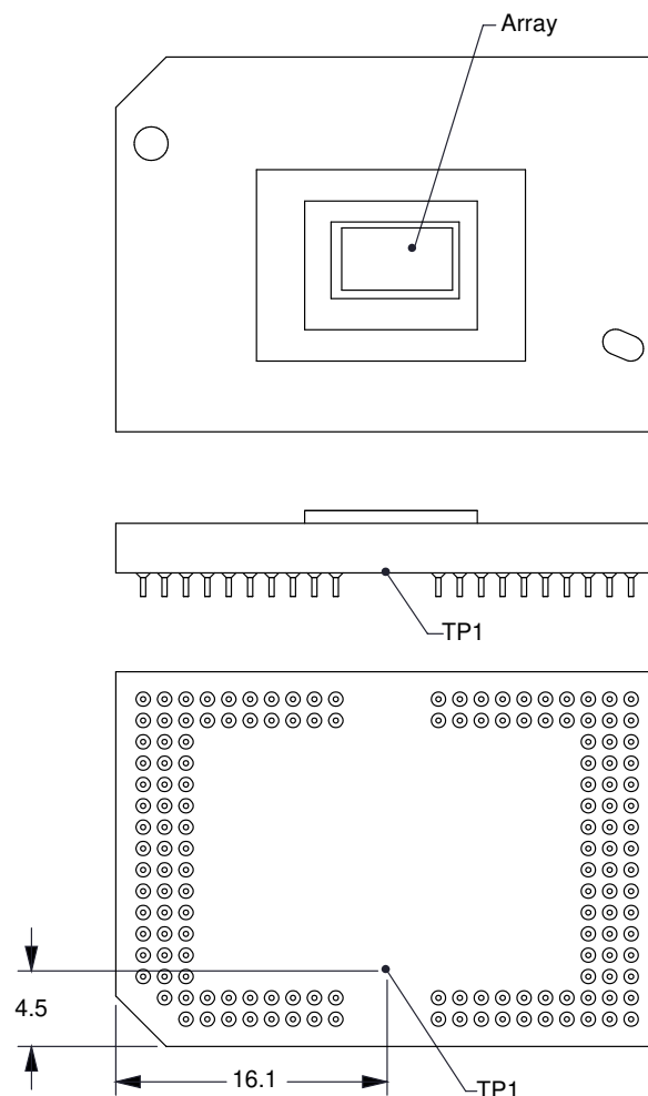
Figure 17. Thermocouple Locations
