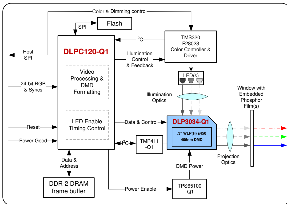
Figure 18. DLP3034-Q1 Reference Design Block Diagram
