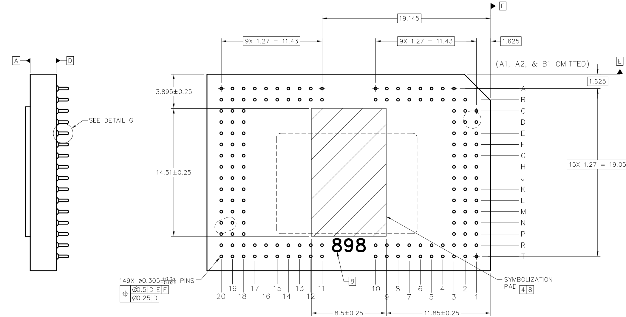
VIEW F-F (SHEET 1) PINS AND SYMBOLIZATION PAD SCALE 8/1
