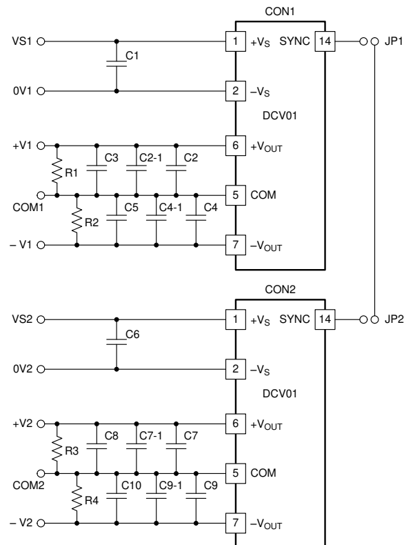
图 11-1. PCB Schematic, P and U Package
