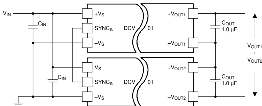
图 8-7. Multiple DCV01 Devices Connected in Series
