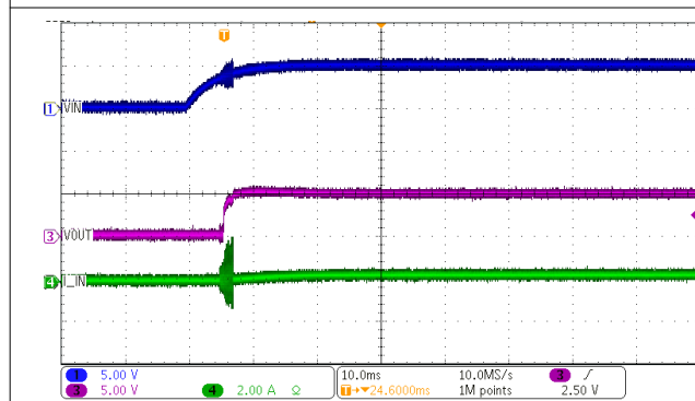
图 8-5. DCV010505P Start-Up at 100% Load
