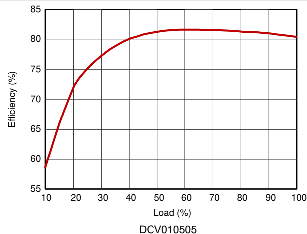
图 7-5. Efficiency versus Load
