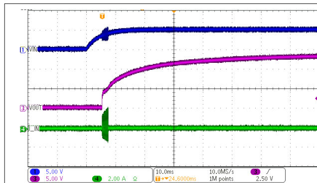
图 8-3. DCV010505P Start-Up at No Load
