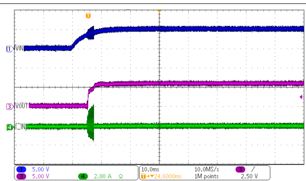
图 8-4. DCV010505P Start-Up at 10% Load
