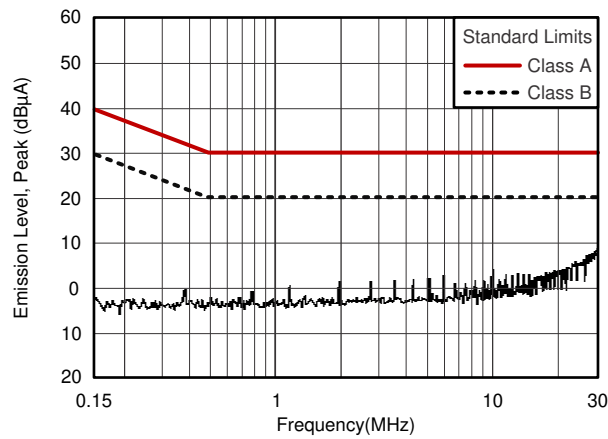
图 7-1. Conducted Emissions
