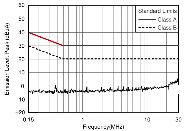
图 7-2. Conducted Emissions
