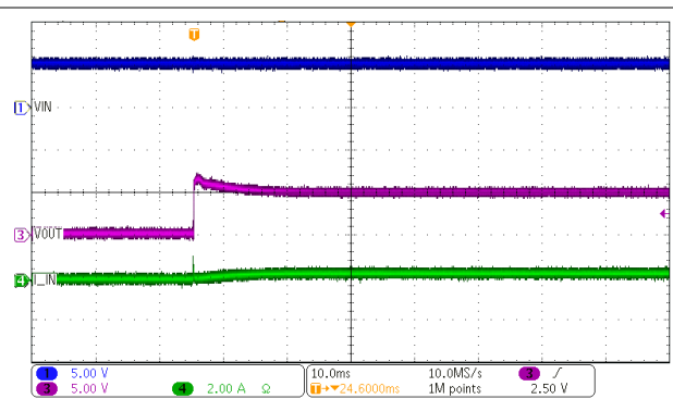
图 8-6. DCV010505P Enable Start-Up at 100% Load
