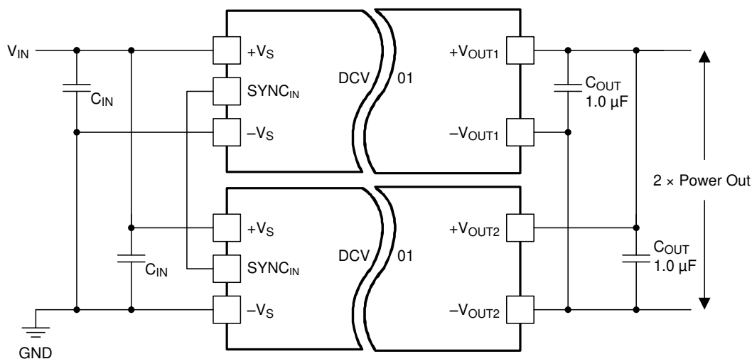
图 8-9. Multiple DCV01 Devices Connected in Parallel
