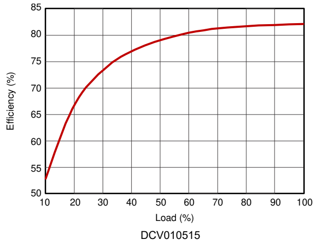
图 7-13. Efficiency versus Load
