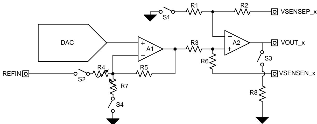
图 128. Simplified Block Diagram of Voltage Output Architecture
