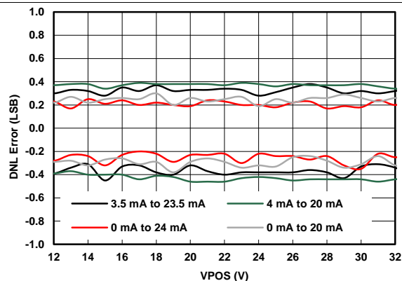
图 16. IOUT Differential Linearity Error vs Power Supplies
