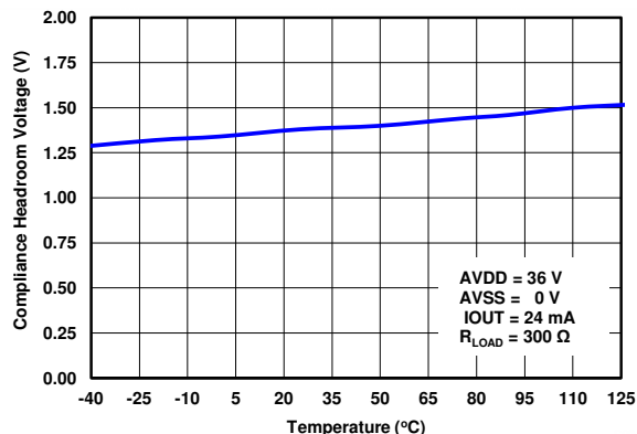
图 7-70. Compliance Headroom Voltage (1) vs Temperature
