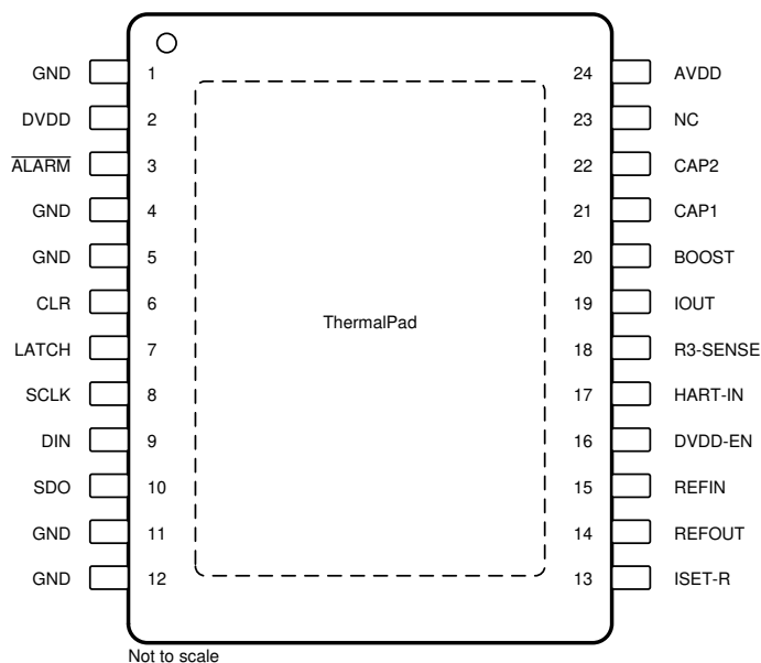
图 6-2. PWP Package, 24-Pin HTSSOP, Top View
