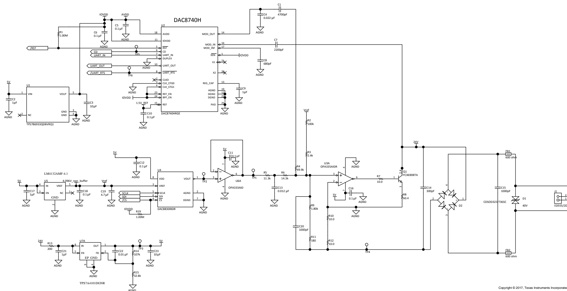
图 34. 2-Wire Transmitter With DAC8740H HART Modem Design Schematic
