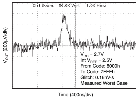
Falling Edge 2.7 V 1-LSB Step
