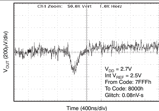
Rising Edge 2.7 V 1-LSB Step
