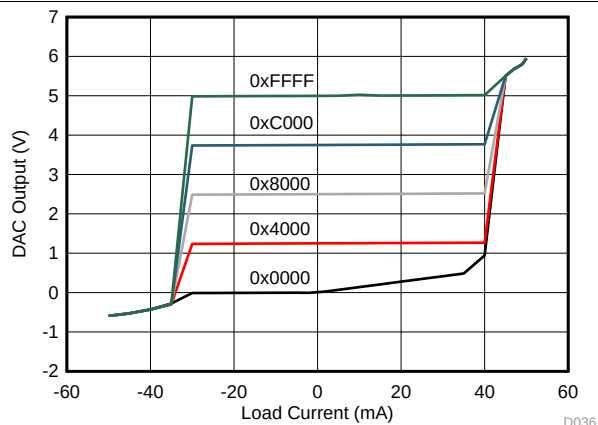
Figure 34. Source and Sink Capability With Gain = \frac{1}{2}
