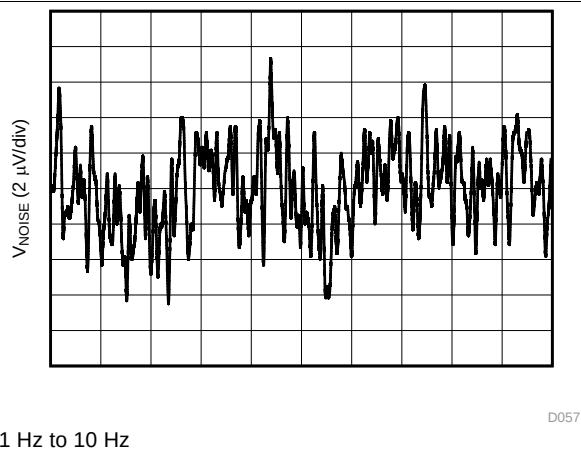
Figure 55. Internal Reference Noise
