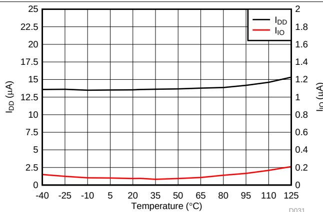
Figure 31. Supply Current and Input Current vs Temperature
