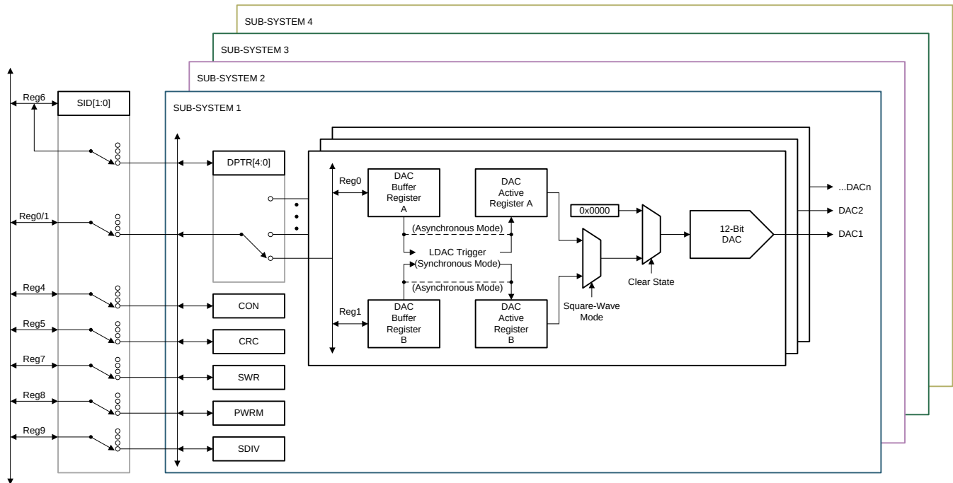
Figure 39. Register Configuration
