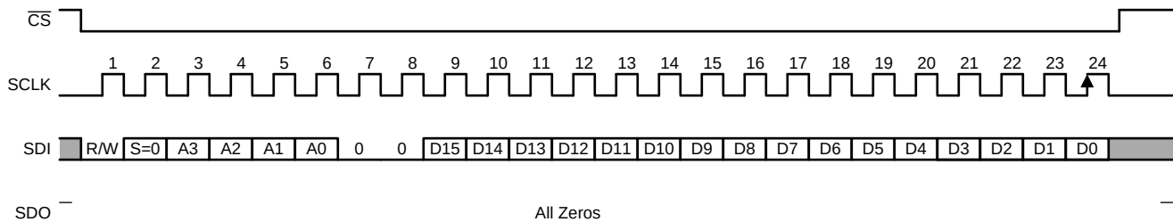
Figure 35. Serial Interface Write Bus Cycle
