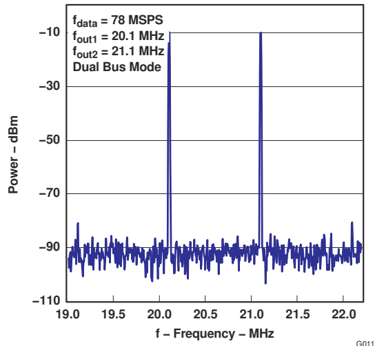
图 6-11. Two-Tone Spectrum
