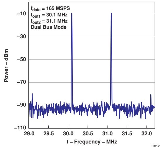
图 6-12. Two-Tone Spectrum
