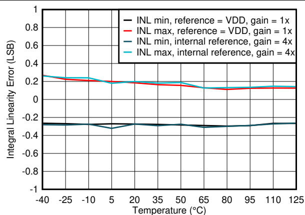
图 6-3. Integral Linearity Error vs Temperature
