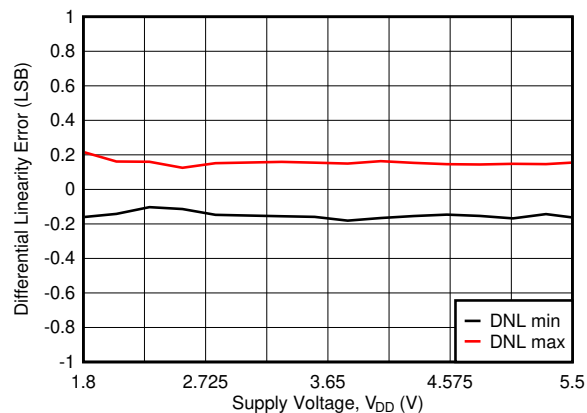
图 6-23. Differential Linearity Error vs Supply Voltage
