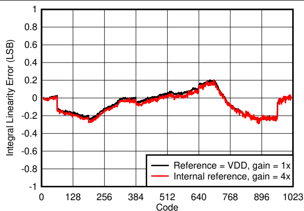
图 6-2. Integral Linearity Error vs Digital Input Code
