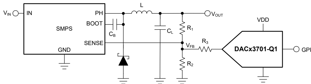
图 8-1. Power-Supply Margining
