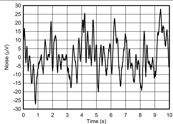
图 6-47. DAC Output Noise: 0.1 Hz to 10 Hz
