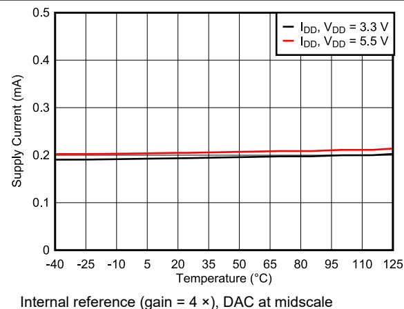
图 6-32. Supply Current vs Temperature
