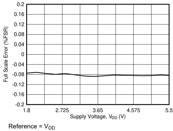
图 6-28. Full-Scale Error vs Supply Voltage
