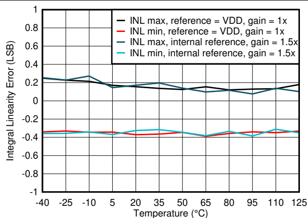
图 6-13. Integral Linearity Error vs Temperature
