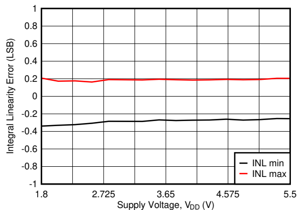
图 6-22. Integral Linearity Error vs Supply Voltage
