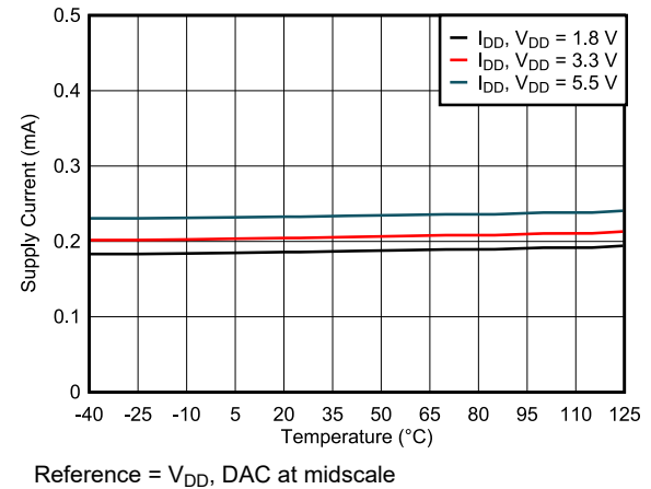
图 6-31. Supply Current vs Temperature
