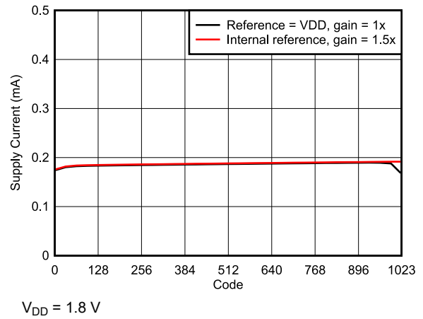
图 6-29. Supply Current vs Digital Input Code
