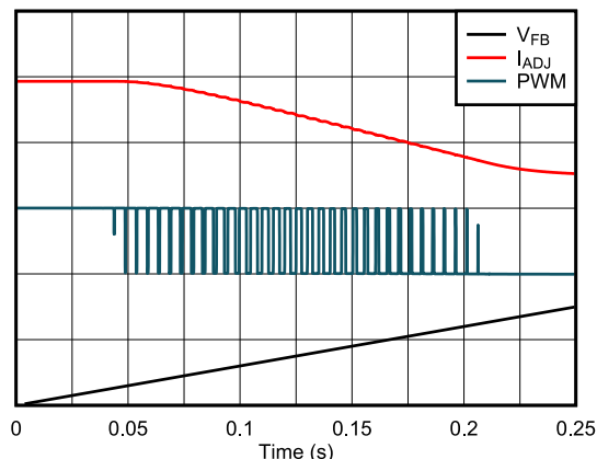
图 8-5. LED Thermal Foldback
