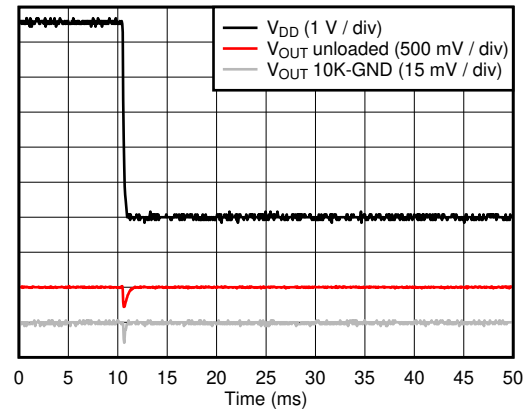
图 6-41. Power-off Glitch
