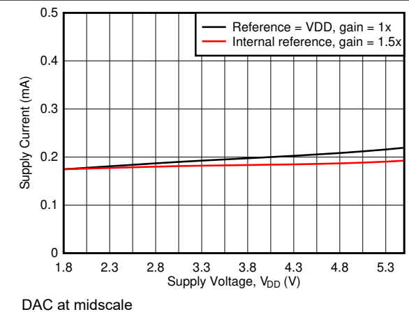
图 6-33. Supply Current vs Supply Voltage
