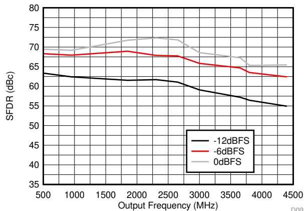
D092 DAC38RF83/93/85
