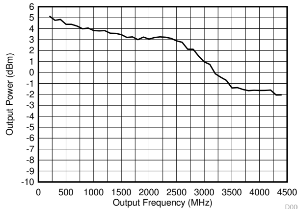
Transformer loss not de-embedded D000 DAC38RF83/93/85
