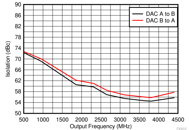
D002 DAC38RF80/90/84
