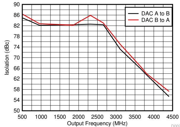
D002 DAC38RF83/93/85
