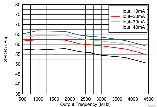
D022 DAC38RF80/90/84
