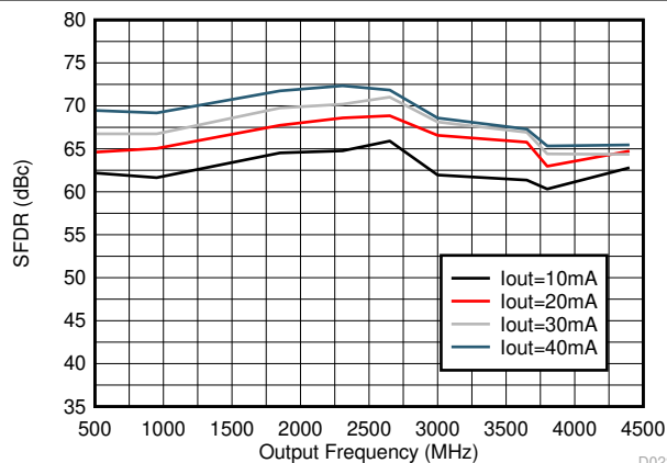
D022 DAC38RF83/93/85
