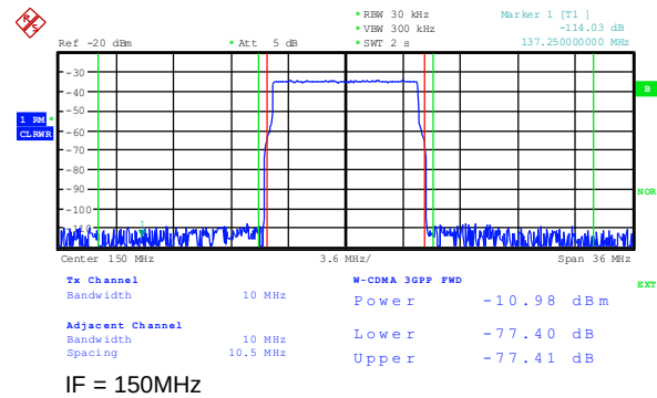
Figure 50. 10MHz Single Carrier LTE Test Mode 3.1
