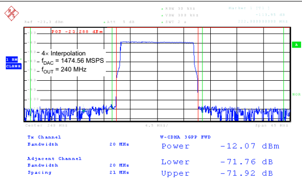
Figure 38. 20-MHz Single-Carrier LTE Test Mode3.1
