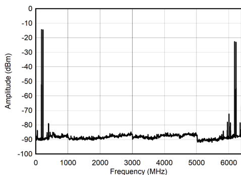
图 6-61. Single Channel RTZ Mode: Dual Tone Spectrum at 200 MHz \pm 25 MHz
