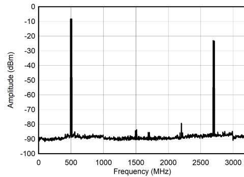
图 6-14. Dual Channel NRZ Mode: Dual Tone Spectrum at 500 MHz ± 10 MHz
