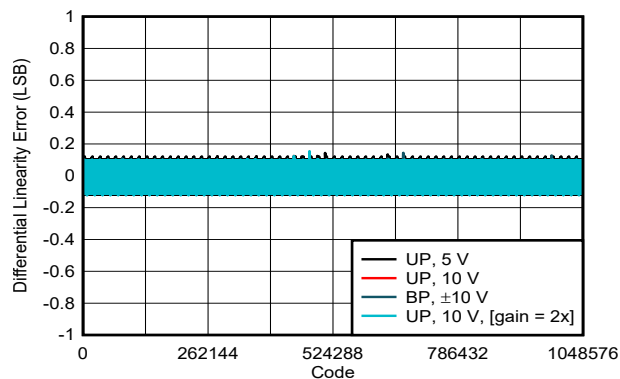
图 6-4. Differential Linearity Error vs Digital Input Code
