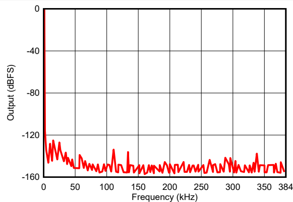
图 6-41. DAC Output Noise Spectral Density
