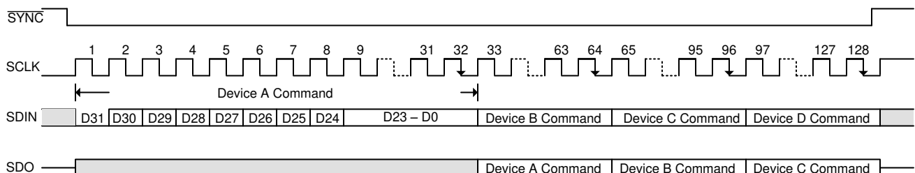
图 7-5. Serial Interface Daisy-Chain Write Cycle
