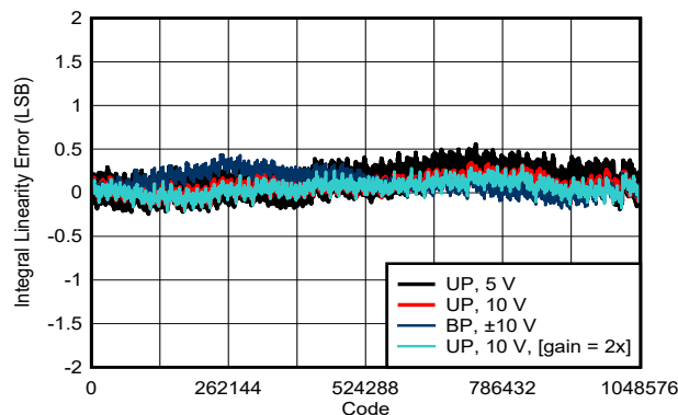
图 6-3. Integral Linearity Error vs Digital Input Code
