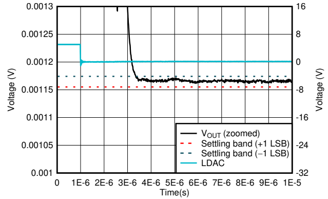
图 6-40. 100 Codes Settling Time, Falling Edge
