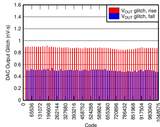
图 6-33. Segment Glitch Impulse, 1-LSB Step
