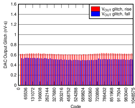
图 6-34. Segment Glitch Impulse, 1-LSB Step
