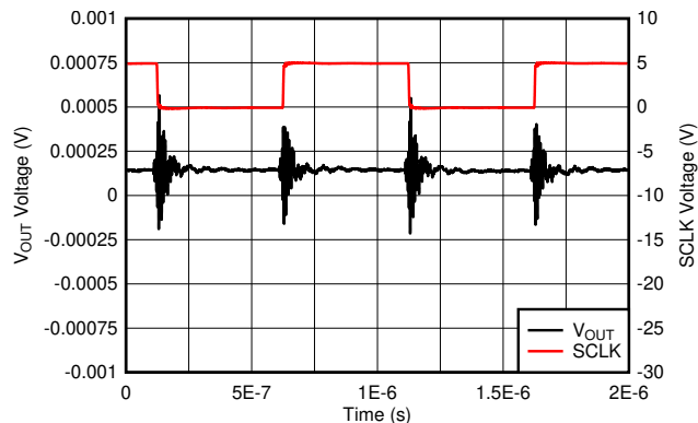
图 6-34. Segment Glitch Impulse, 1-LSB Step
