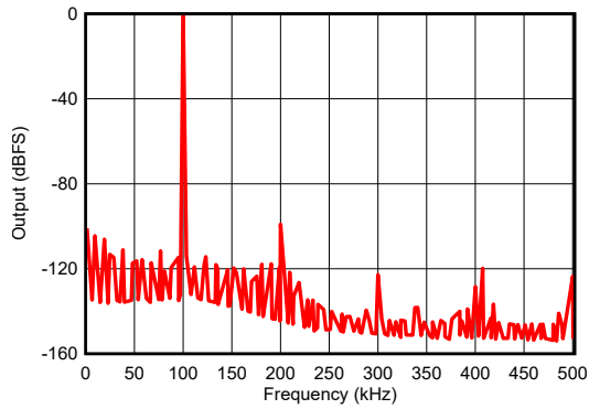
图 6-45. 100-kHz Spectrum vs Frequency
