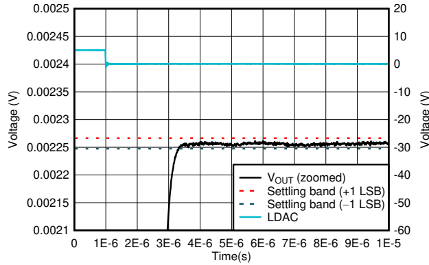
图 6-39. 100 Codes Settling Time, Rising Edge
