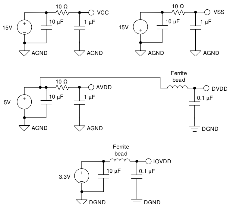
图 9-5. Power-Supply Decoupling
