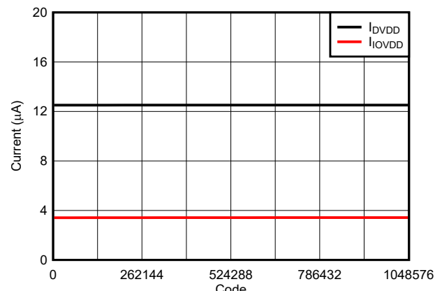
V_{REFPF} = 10\text{ V} , V_{REFNF} = 0\text{ V} 图 6-20. Supply Current ( DV_{DD} and IOV_{DD} ) vs Digital Input Code
