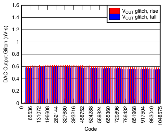
图 6-33. Segment Glitch Impulse, 1-LSB Step
