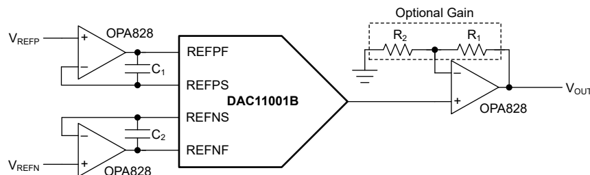
图 8-7. Arbitrary Waveform Generation
