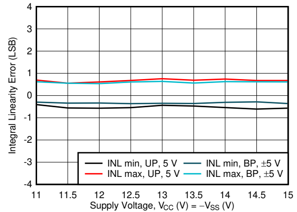
图 6-10. Integral Linearity Error vs Supply Voltage
