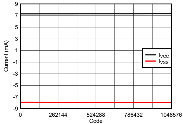
图 6-21. Supply Current ( V_{CC} and V_{SS} ) vs Digital Input Code
