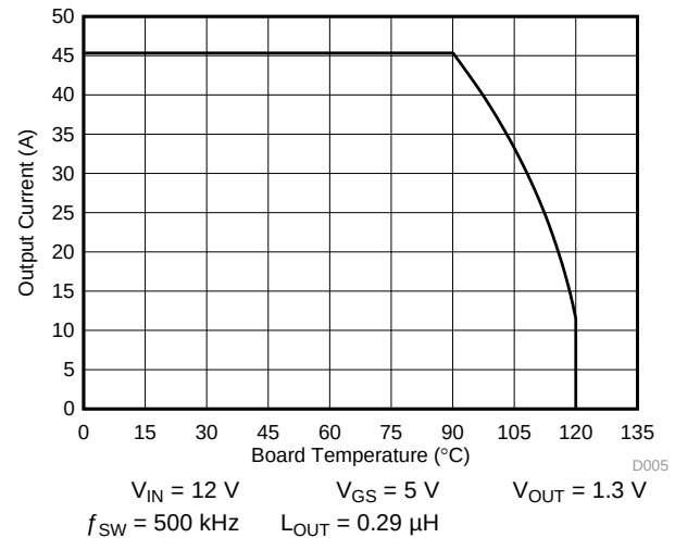
图 4. Typical Safe Operating Area (SOA)
