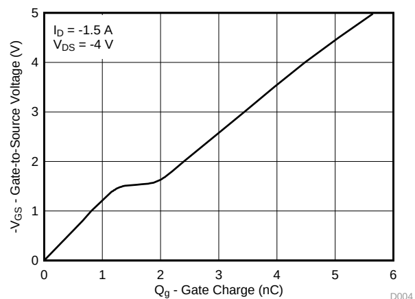
栅极电荷
