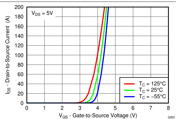
图 4-3. Transfer Characteristics
