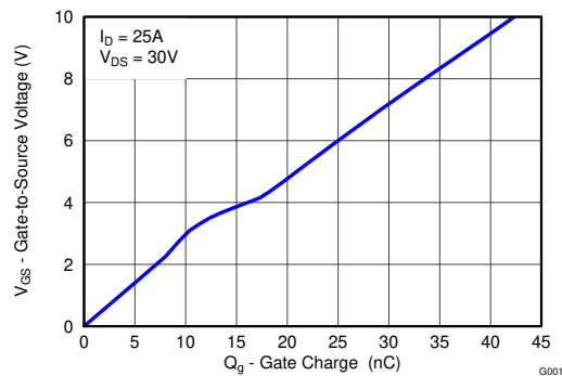
栅极电荷
