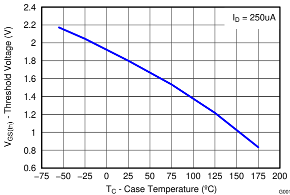
图 3-6. Threshold Voltage vs Temperature
