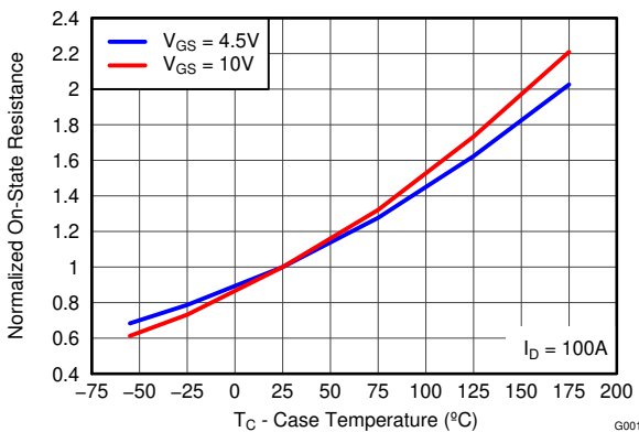
图 3-8. Normalized On-State Resistance vs Temperature
