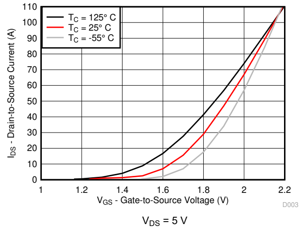
图 4-3. Transfer Characteristics
