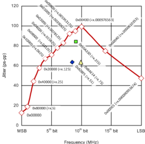
Figure 4. Fractional Divider Bit Selection Impact on Jitter ( f_{ERAC} = 300 \text{ MHz} )
