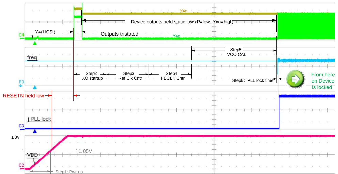
Figure 60. Power-Up Time
