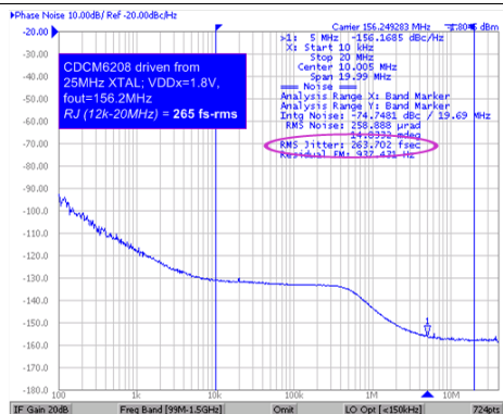
Figure 2. Typical Device Output Phase Noise and Jitter for 25 MHz
