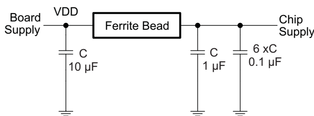
Figure 24. Power-Supply Decoupling
