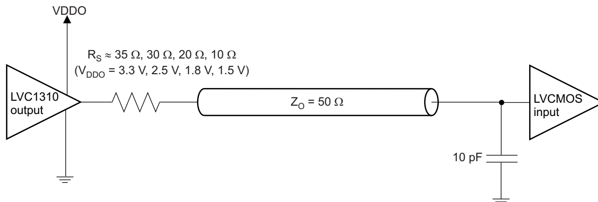
Figure 9. LVC MOS Output DC Configuration: Typical Application Load
