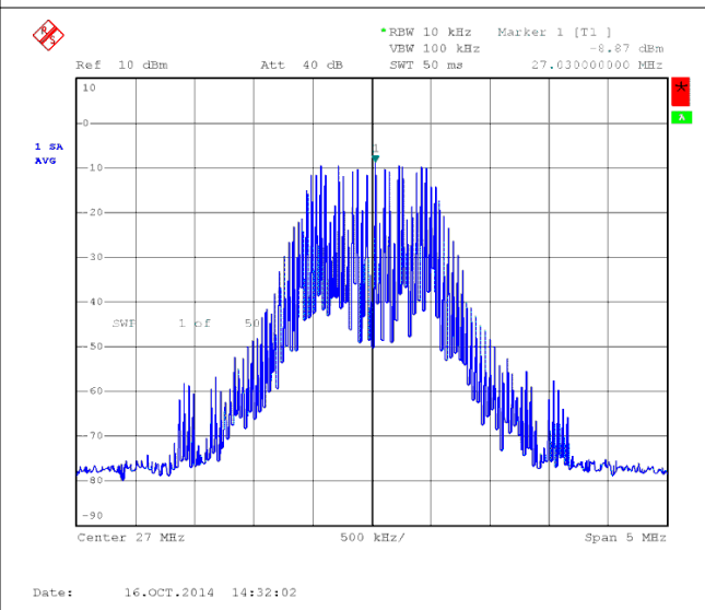
图 9-9. Output Spectrum With SSC On, 2% Center
