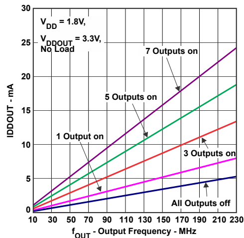
图 5-2. CDCE937 Output Current vs Output Frequency
