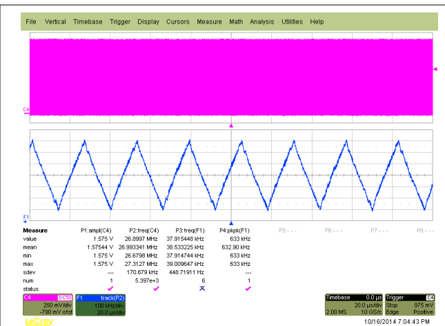
图 9-7. f_{out} = 27\text{MHz} , VCO frequency > 175MHz, SSC (1%, center)
