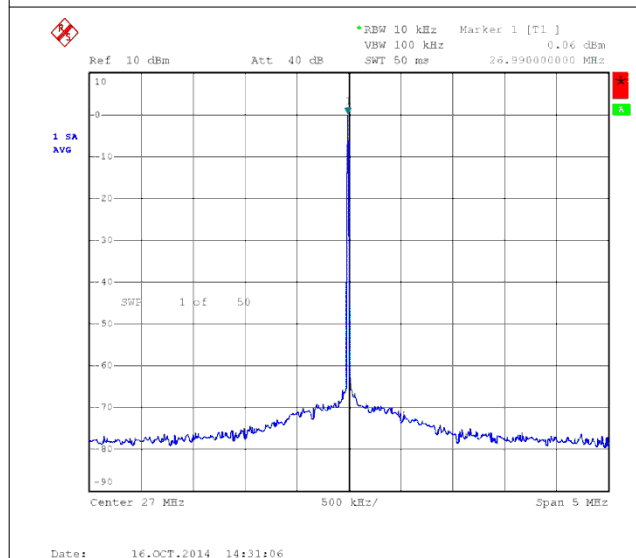
图 9-8. Output Spectrum With SSC Off
