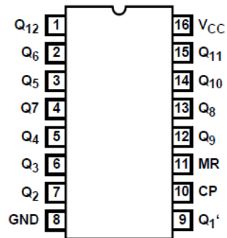
J, D, or N package 16-Pin CDIP, SOIC, or PDIP Top View
