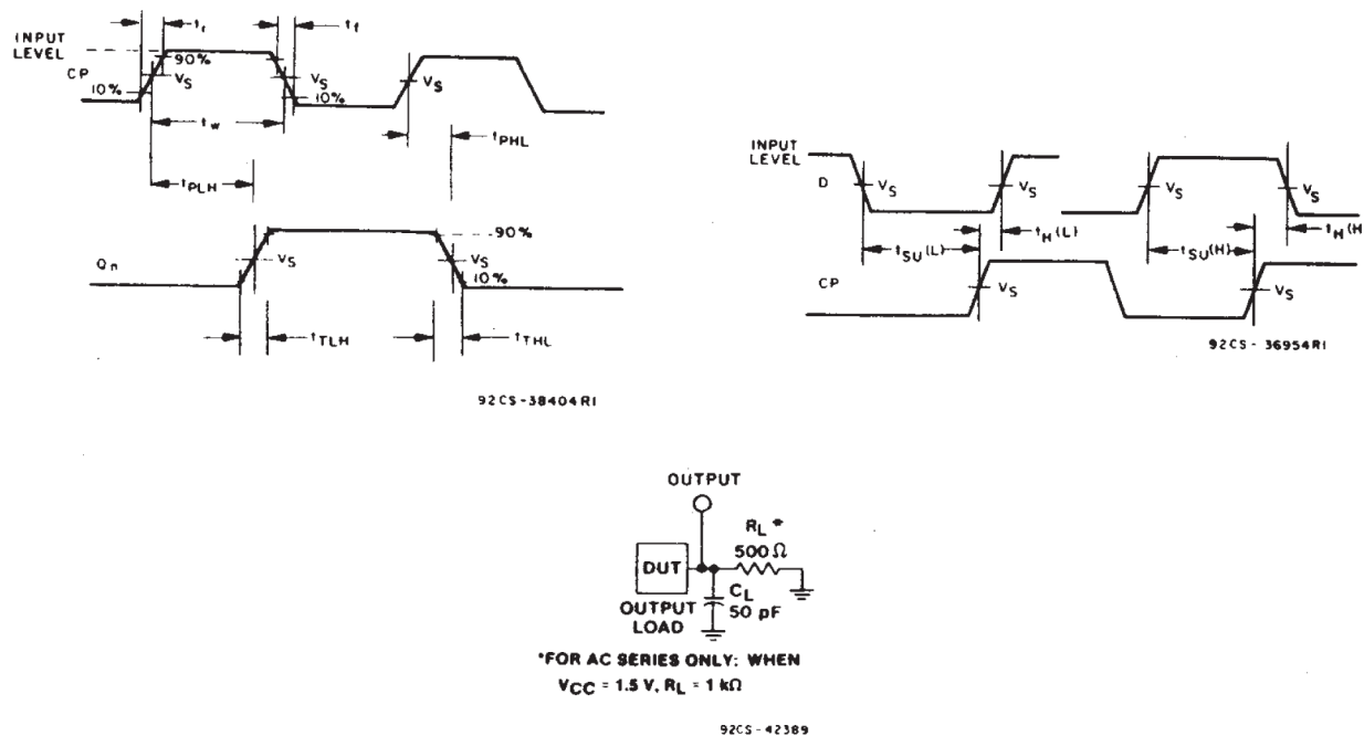
图 5-3. Propagation Delay Times and Test Circuit.
