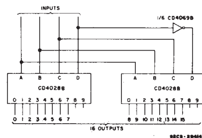
Fig. 13 – Code conversion circuit.
