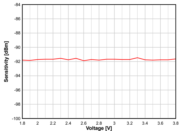
图 8-14. Sensitivity versus Supply Voltage (VDDS) (WBMS, 2.44 GHz, DCDC off)
