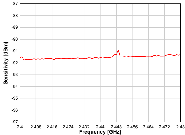
图 8-11. Sensitivity versus Frequency (WBMS, 2.44 GHz)
