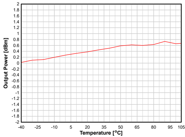
图 8-15. Output Power vs. Temperature (WBMS, 2.44 GHz, 0dBm)
