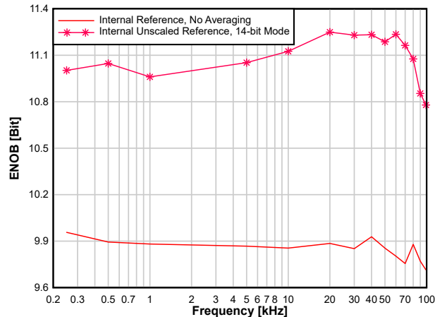
图 8-21. ENOB versus Input Frequency
