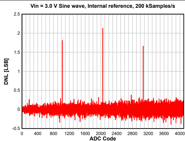
图 8-24. DNL versus ADC Code
