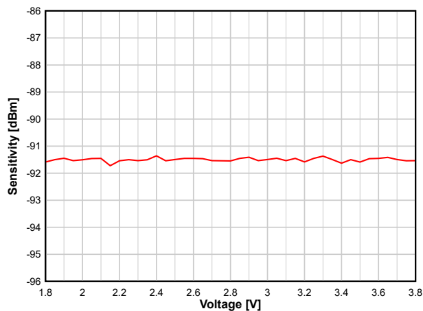
图 8-13. Sensitivity versus Supply Voltage (VDDS) (WBMS, 2.44 GHz)
