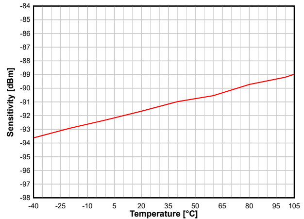
图 8-12. Sensitivity versus Temperature (WBMS, 2.44 GHz)
