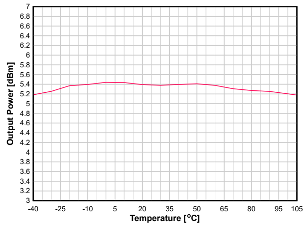
图 8-16. Output Power vs. Temperature (WBMS, 2.44 GHz, +5dBm)
