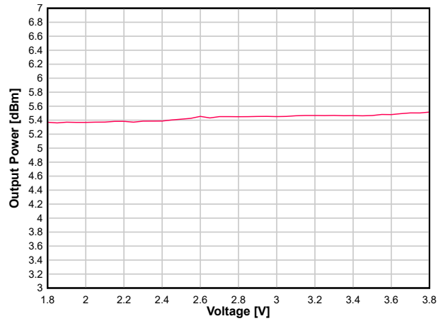
图 8-18. Output Power vs. Supply Voltage (VDDS) (WBMS, 2.44 GHz, +5dBm)
