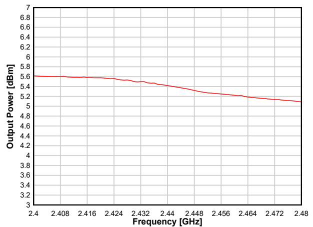
图 8-20. Output Power vs. Frequency (WBMS, +5dBm)
