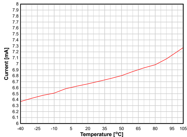
图 8-7. RX Current versus Temperature (WBMS, 2.44 GHz)
