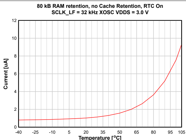
图 8-5. Standby Mode (MCU) Current vs. Temperature
