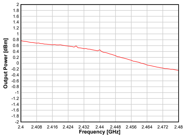
图 8-19. Output Power vs. Frequency (WBMS, 0dBm)
