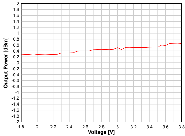
图 8-17. Output Power vs. Supply Voltage (VDDS) (WBMS, 2.44 GHz, 0dBm)
