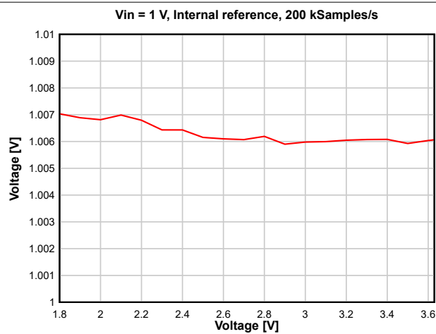
图 8-26. ADC Accuracy versus VDD5
