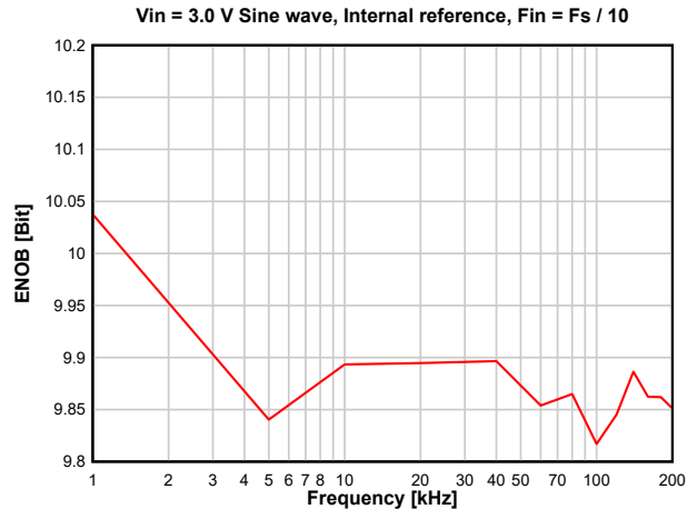
图 8-22. ENOB versus Sampling Frequency
