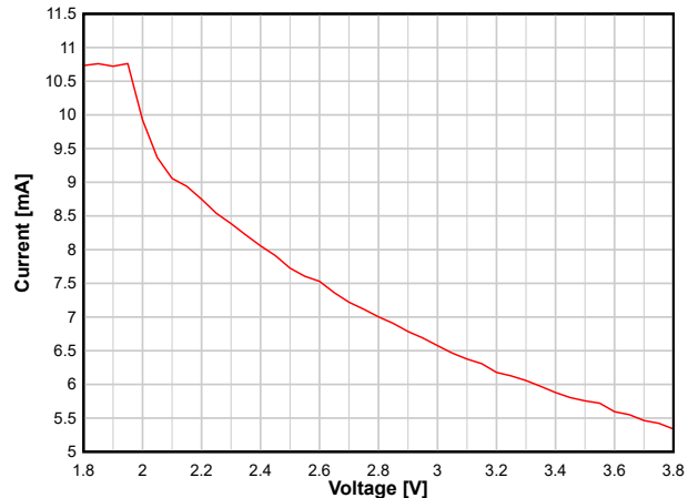
图 8-8. RX Current versus Supply Voltage (VDDS) (WBMS, 2.44 GHz)
