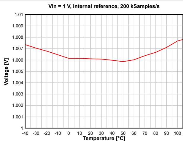
图 8-25. ADC Accuracy versus Temperature
