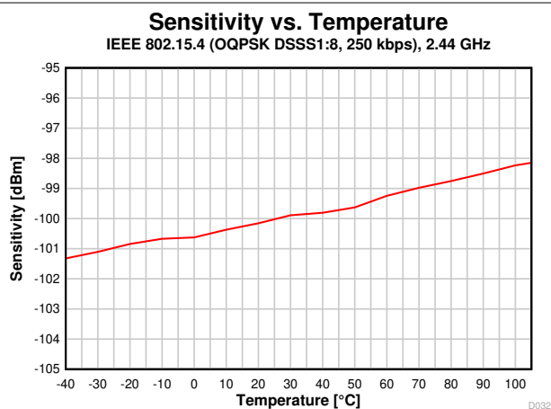
图 7-13. Sensitivity vs. Temperature (250 kbps, 2.44 GHz)
