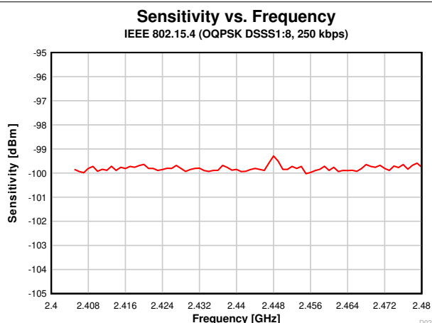
图 7-11. Sensitivity vs. Frequency (250 kbps, 2.44 GHz)
