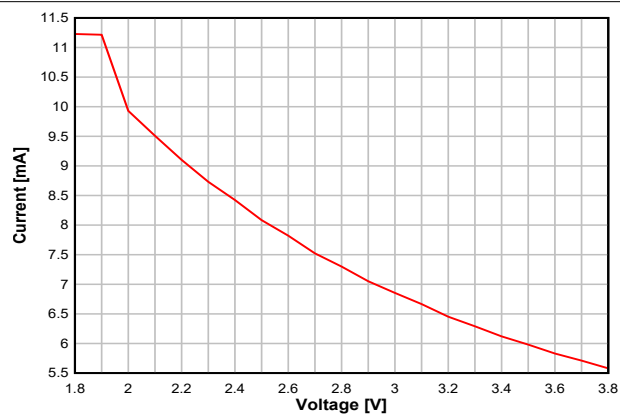
图 7-7. RX Current vs. Supply Voltage (VDD) (BLE 1Mbps, 2.44GHz)
