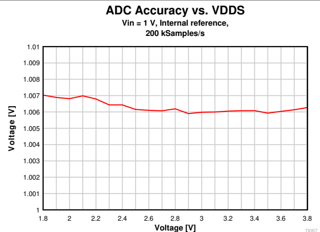
图 8-38. ADC Accuracy vs. Supply Voltage (VDD)
