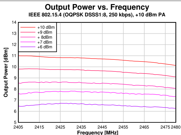
图 8-32. Output Power vs. Frequency (250 kbps, +10 dBm PA)
