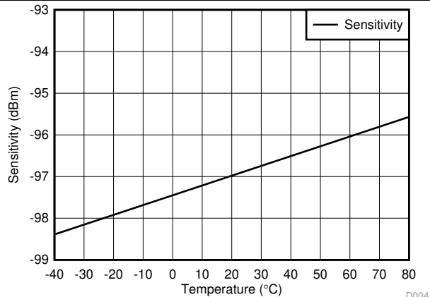
Figure 5-4. Bluetooth low energy Sensitivity vs Temperature D004
