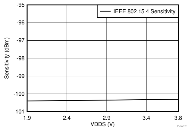
Figure 5-7. IEEE 802.15.4 Sensitivity vs Supply Voltage (VDD) D007
