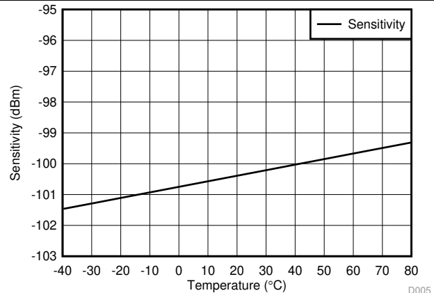
Figure 5-5. IEEE 802.15.4 Sensitivity vs Temperature D005
