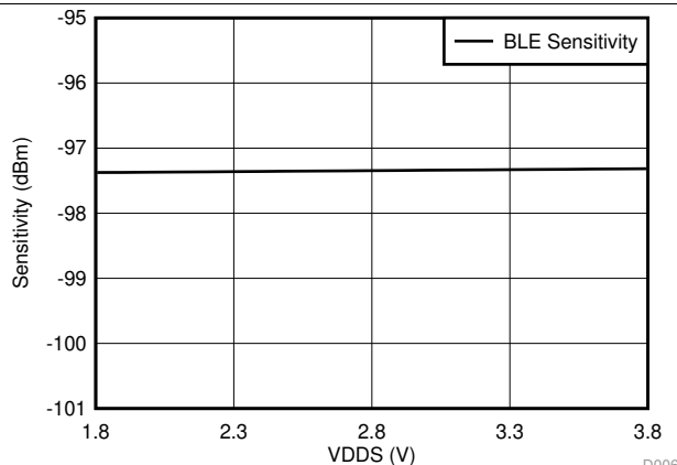
Figure 5-6. Bluetooth low energy Sensitivity vs Supply Voltage (VDD) D006
