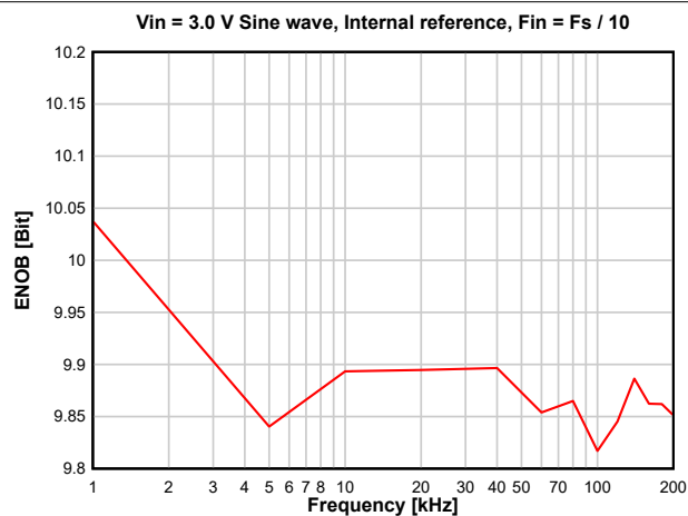
图 8-23. ENOB versus Sampling Frequency
