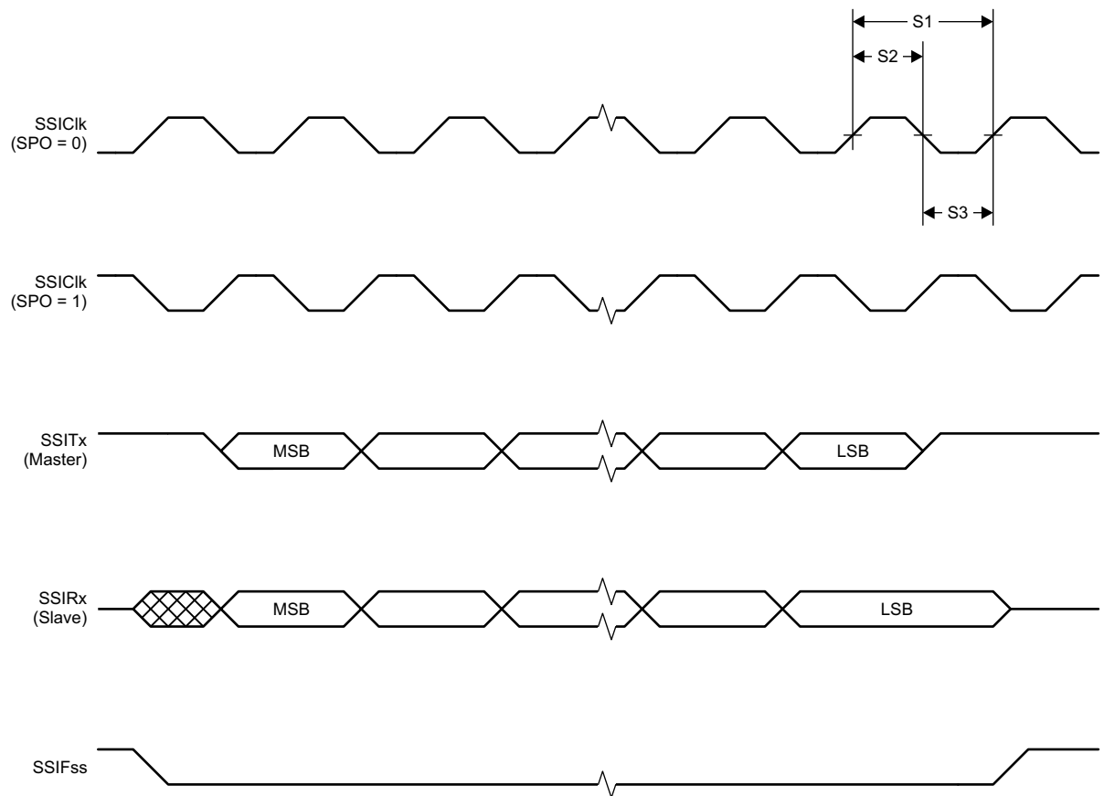
图 8-3. SSI Timing for SPI Frame Format (FRF = 00), With SPH = 1
