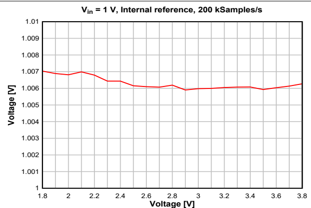
图 8-25. ADC Accuracy vs. Supply Voltage (VDDS)
