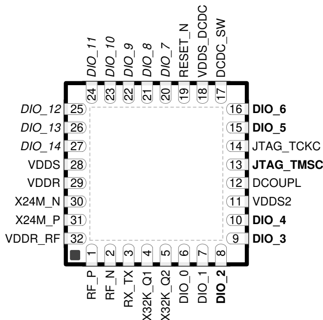
图 7-2. RHB Package 32-Pin VQFN (5-mm x 5-mm) Pinout, 0.5-mm Pitch
