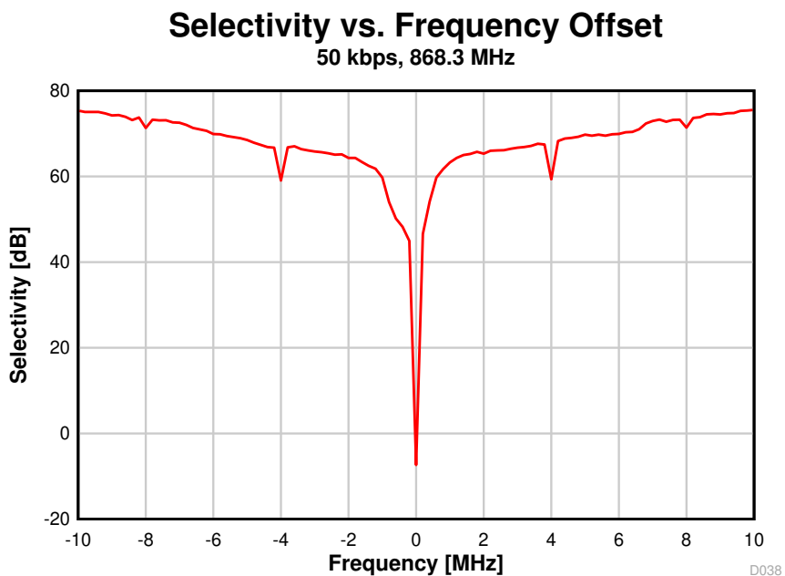
图 8-28. Selectivity vs. Frequency Offset (50 kbps, 868.3 MHz)
