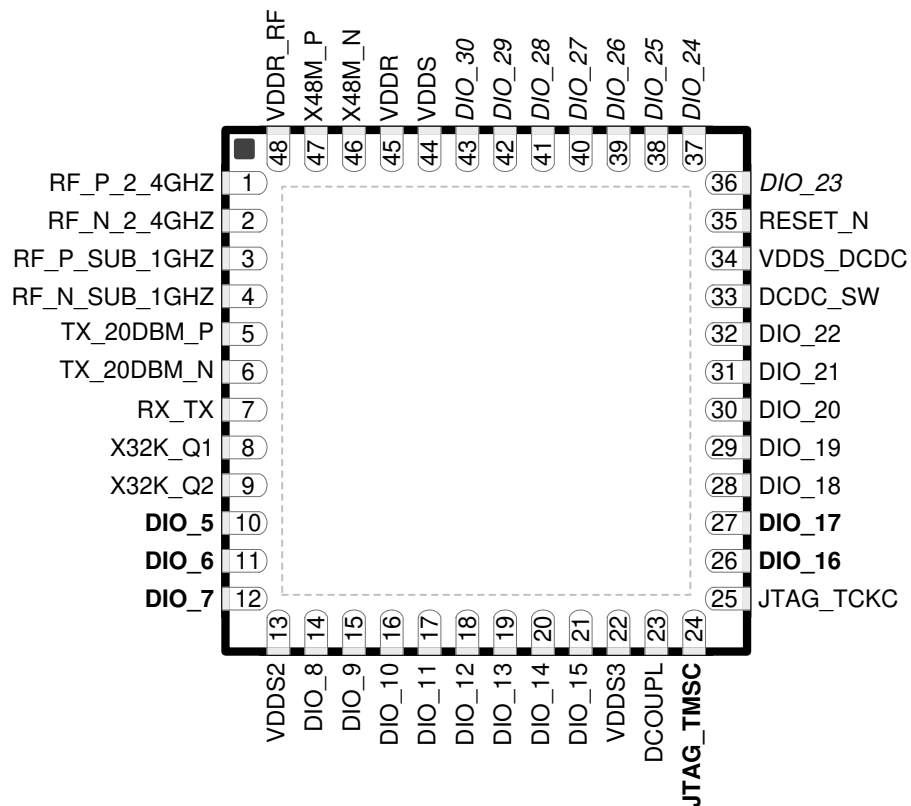
图 6-1. RGZ (7-mm x 7-mm) Pinout, 0.5-mm Pitch (Top View)
