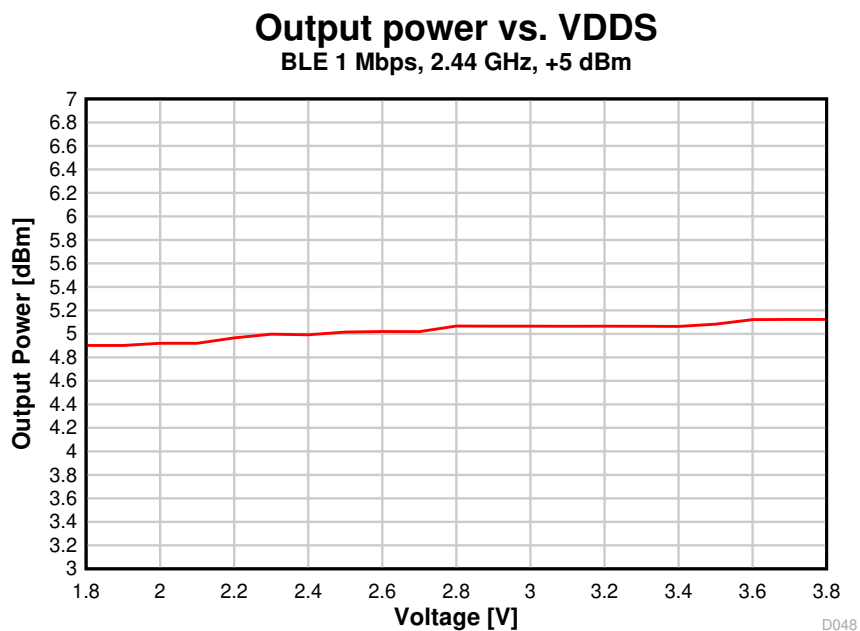
图 8-48. Output Power vs. Supply Voltage (VDDS) (BLE 1 Mbps, 2.44 GHz, +5 dBm)
