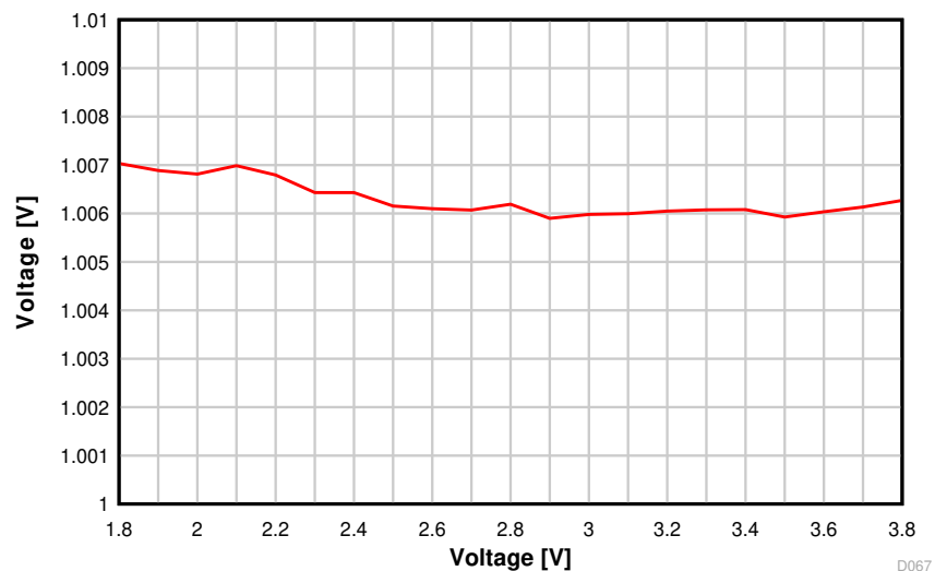
图 8-63. ADC Accuracy vs. Supply Voltage (VDDS)
