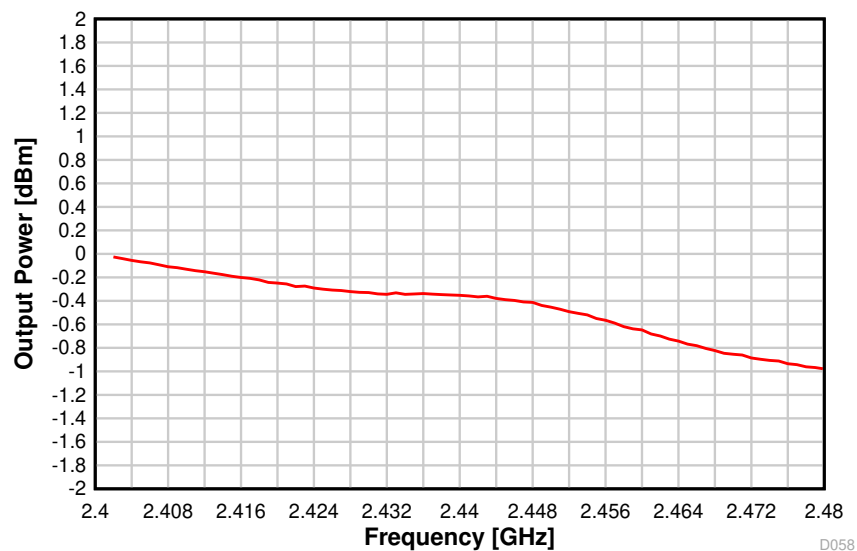
图 8-54. Output Power vs. Frequency (BLE 1 Mbps, 2.44 GHz)
