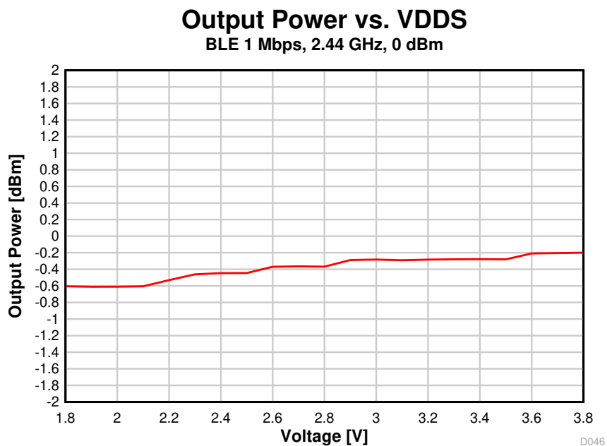
图 8-47. Output Power vs. Supply Voltage (VDDS) (BLE 1 Mbps, 2.44 GHz)
