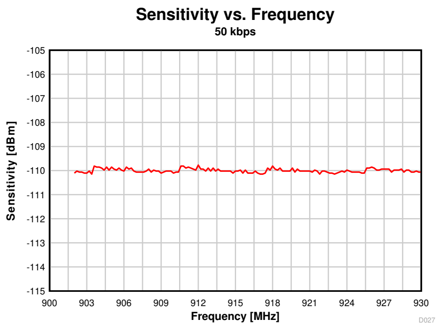
图 8-24. Sensitivity vs. Frequency (50 kbps, 915 MHz)
