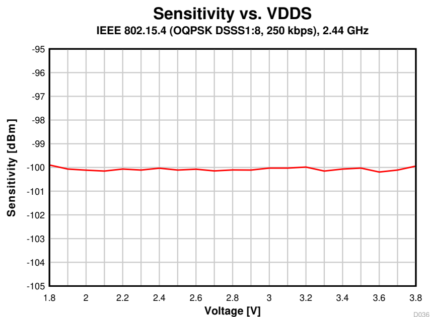
图 8-33. Sensitivity vs. Supply Voltage (VDD5) (250 kbps, 2.44 GHz)
