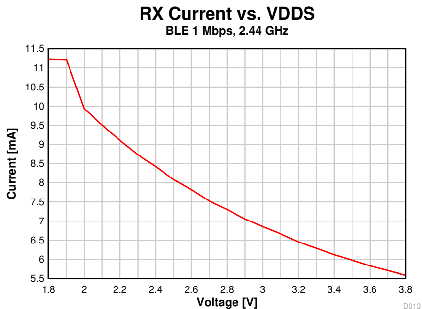
图 8-11. RX Current vs. Supply Voltage (VDD5) (BLE 1 Mbps, 2.44 GHz)
