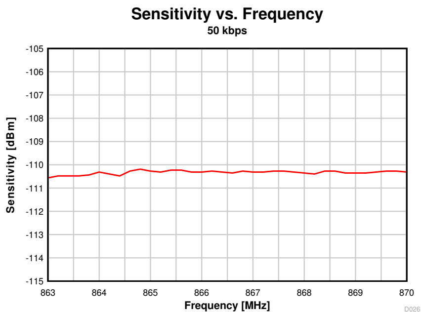
图 8-23. Sensitivity vs. Frequency (50 kbps, 868 MHz)
