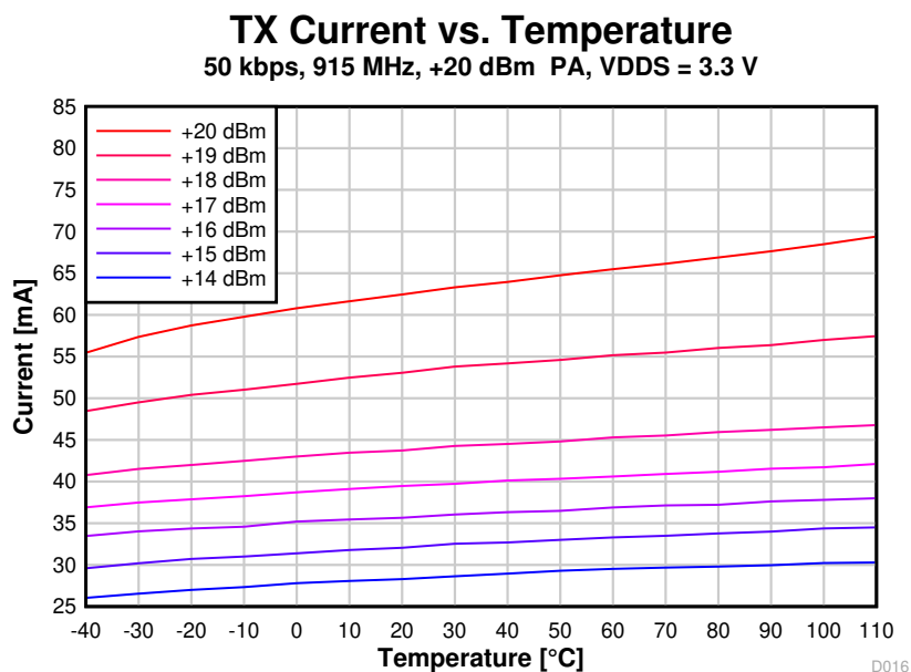
图 8-14. TX Current vs. Temperature (50 kbps, 915 MHz, VDDS = 3.3 V)
